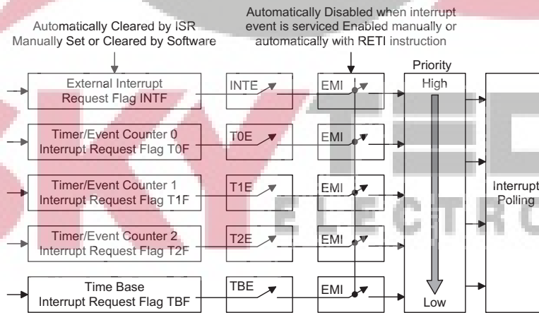
Interrupt Scheme
