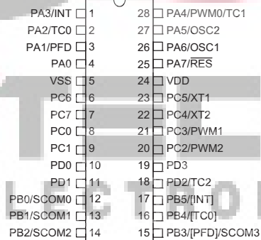
HT48R067 28 SKDIP-A/SOP-A/SSOP-A
