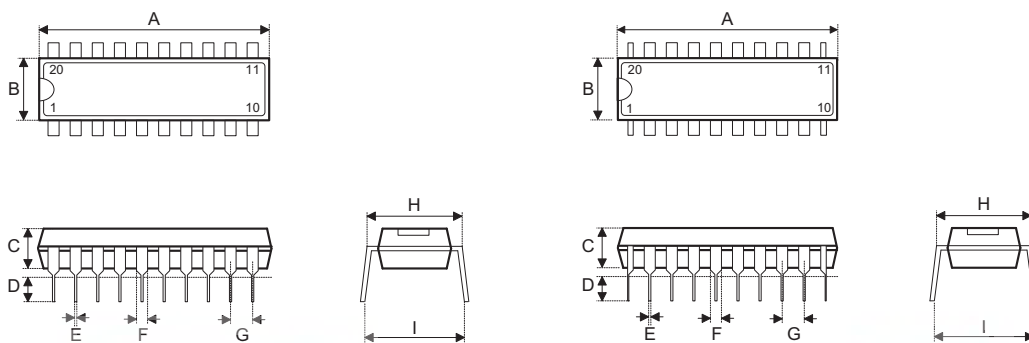
Fig1. Full Lead Packages
