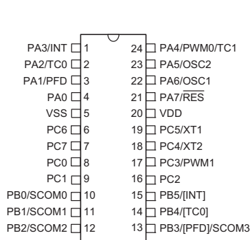
HT48R0662 24 SKDIP-A/SOP-A/SSOP-A
