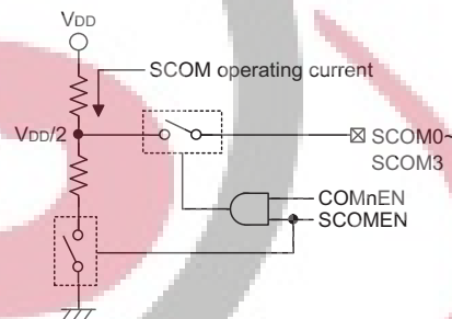
SCOM Circuit
